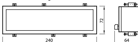
Dimensional drawing D
